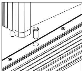
Figure 2g (In-swing sill)
